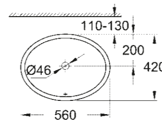
39 423 000 Undercounter basin 55 cm
