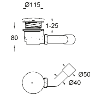
49 534 000* Waste set horizontal for Universal shower trays
