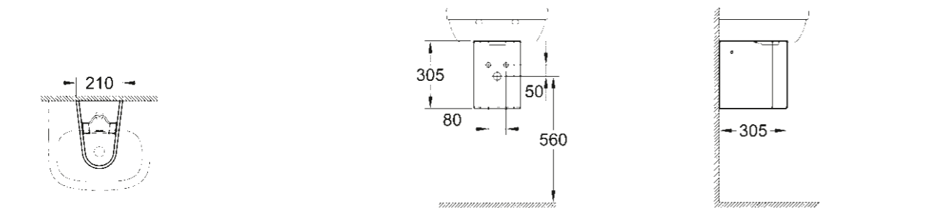
39 325 000 Semi pedestal for handrinse basin 45 cm
