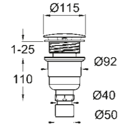
49 533 000* Waste set vertical for Universal shower trays
