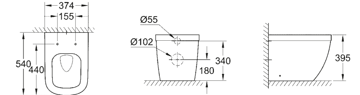
39 339 000 39 339 00H* Floorstanding WC back to wall rimless
