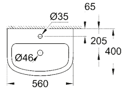
39 422 000 Drop in basin 55 cm
