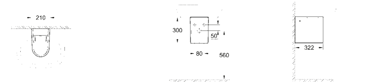
39 201 000 Semi pedestal for wash basins
