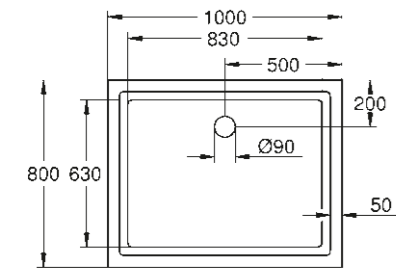
39 306 000* Universal shower tray 80 cm x 100 cm
