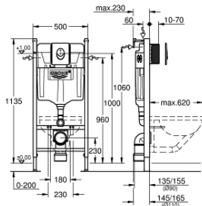
38 745 001 Rapid SL 3-in-1 Set for WC, 1,13 m Installation Height
