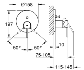
24 060 003 Single-lever mixer with 2-way diverter
