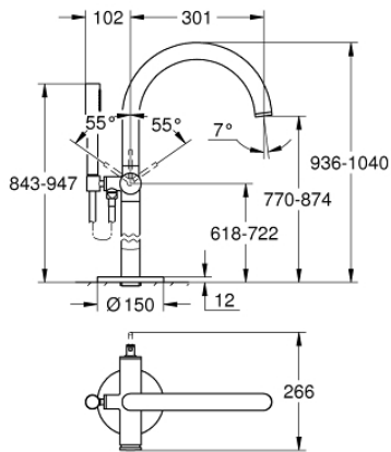
32 653 003 32 653 DC3 32 653 AL3 Single-lever bath mixer, floor mounted
