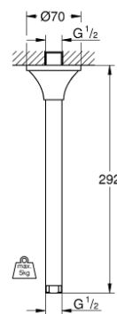
27 982 000 RAINSHOWER GRANDERA SHOWER Arm ceiling 292 mm
