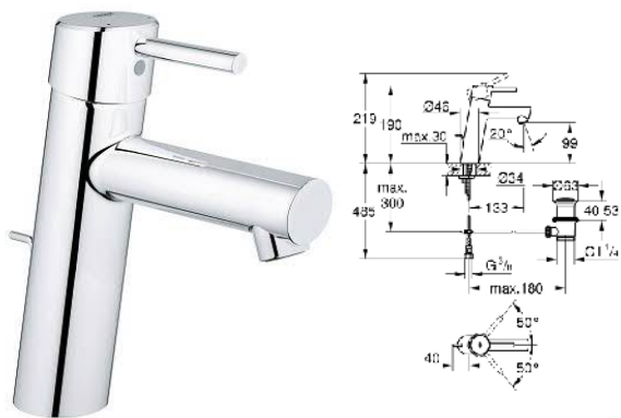
23 450 001 Basin mixer 1/2 M-Size
