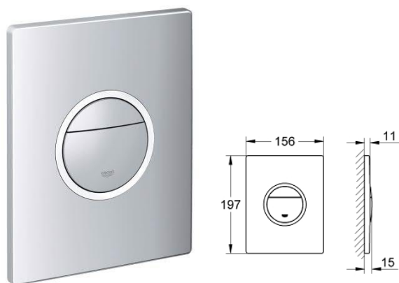
Arena Cosmopolitan S Flush plate
