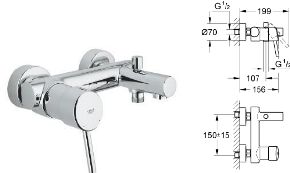
32 211 001 Single-lever bath/shower mixer 1/2
