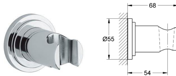
28 690 000 Sena Wall hand Shower holder
