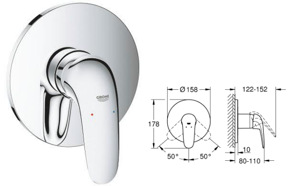
24 046 003 — 24 046 LS3 Single-lever shower mixer trim
