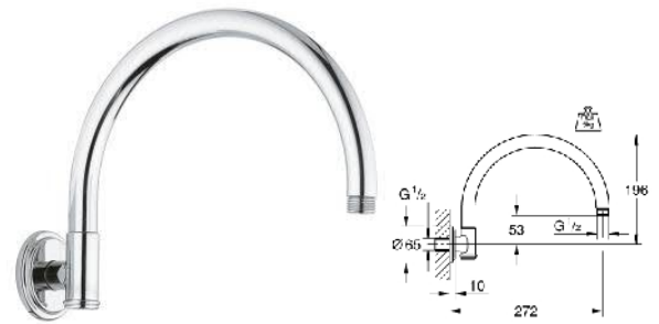
28 384 000 Rainshower rustic shower arm 272 mm
