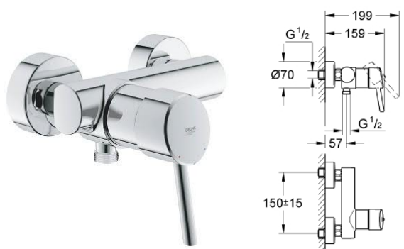
19 573 002 2-hole basin mixer M-Size
