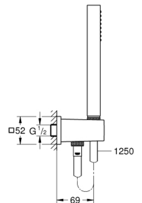
26 405 000 Euphoria Cube Stick Wall holder set 1 spray
