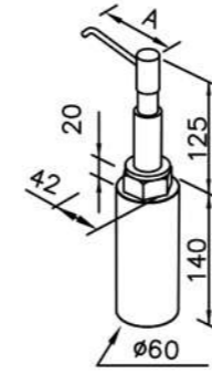
Soap Dispenser 6759-26-80CP A:81mm 6759-26-81CP A:163mm
