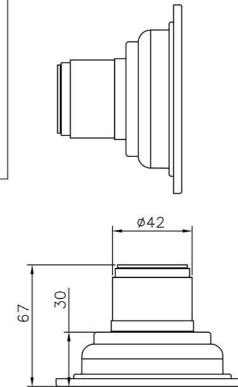
Floor Drain 100x100 mm 0305-21-79S1
