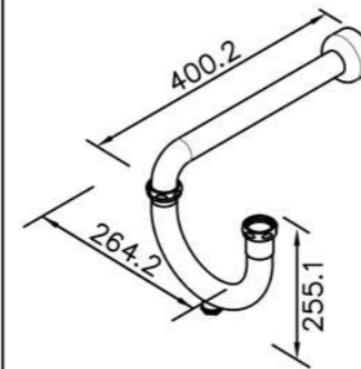
U-Trap W / Cleanout 6119-AU-80CP 1 1/2" 6119-BU-80CP 1 1/4"
