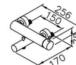
6768-94-80CP Bath / Shower Mixer Body
