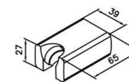
7909-9C-80CP Adjustable Wall Bracket
