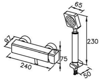
6909-93-81CP Shower Mixer W / Hand Shower W / Hose 150cm & Wall Bracket
