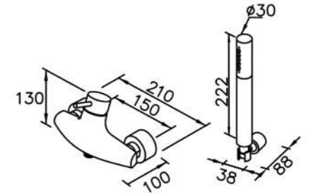
6780-93-81CP Shower Mixer W / Hand Shower & Hose & Wall Bracket
