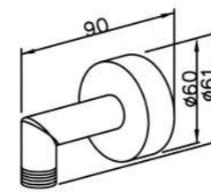
6880-AD-80CP Wall Supply G1/2
