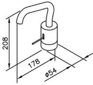
6777-90-80CP Basin Faucet
