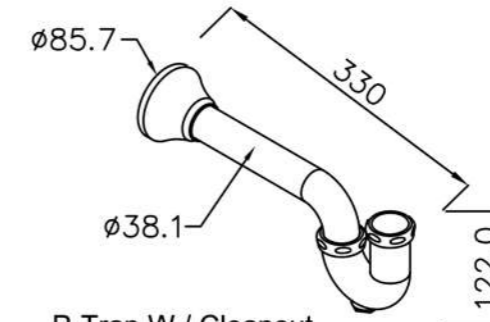
P-Trap W / Cleanout 6119-A3-80CP 1 1/2" 6119-B3-80CP 1 1/4"
