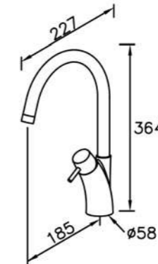
6780-96-80CP Kitchen Faucet
