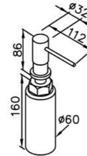
Soap Dispenser 6770-26-80S1 Stainless Steel 6771-26-80CP Brass
