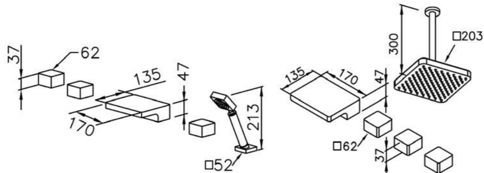
6909-M2-80CP Three-Handle Bathtub Faucet W / Hand Shower & Diverter
