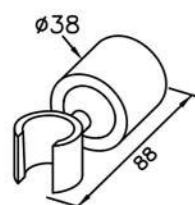
6767-9C-80S1 Wall Bracket
