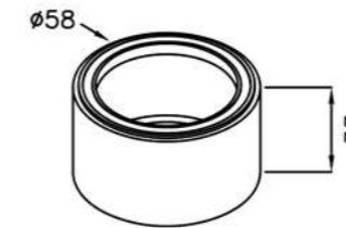
6502-CB-80CP Insert Spacer O.D 58*H33mm
