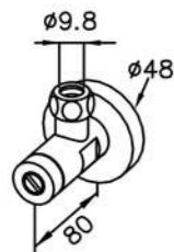
6874-Y8-81CP 1/2" IPS x 3/8" O.D.
