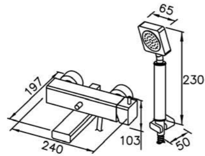
6909-94-81CP Bath / Shower Mixer W / Hand Shower W / Hose 150cm & Wall Bracket
