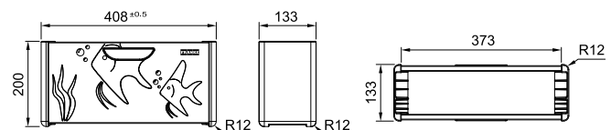
Active Plus Soap Dispenser Dimensions
