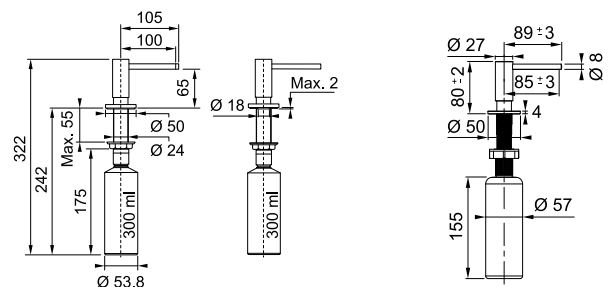
Active Plus Soap Dispenser Dimensions
