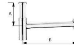
T-Trap 6502-TT-80CP A:170 B:340mm 6502-TT-81CP A:170 B:485mm
