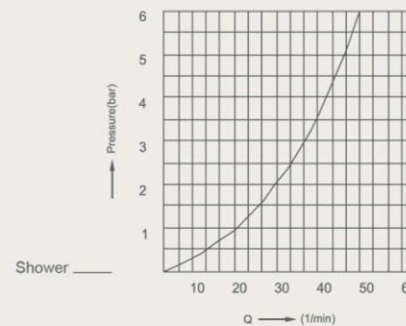
Pressure loss curve without downstream resistance.
