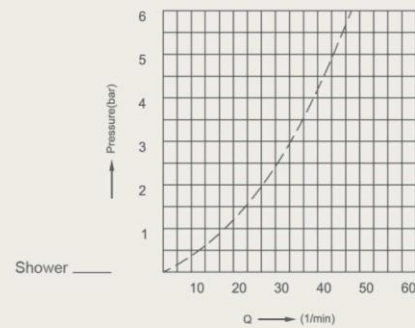
Pressure loss curve without downstream resistance.
