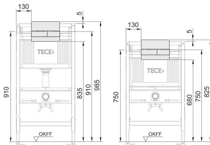
980 mm / 820 mm
