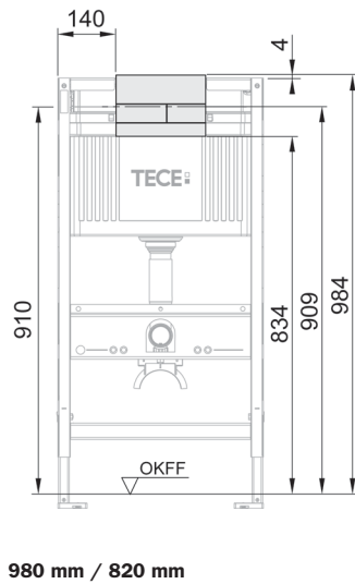
980 mm / 820 mm
