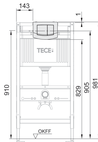
980 mm / 820 mm
